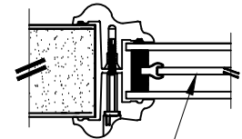
DECORATIVE INSERT
