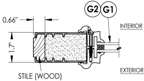
1 HORIZONTAL CROSS SECTION Lip Lite Glazing
